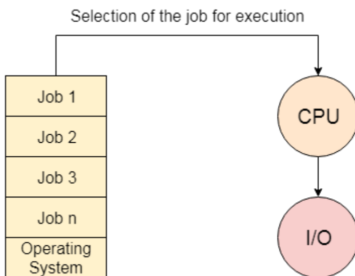
Job Queue
